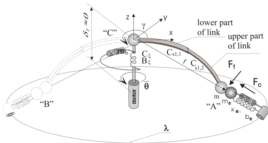
Figure 4: Mechanism robotic.
