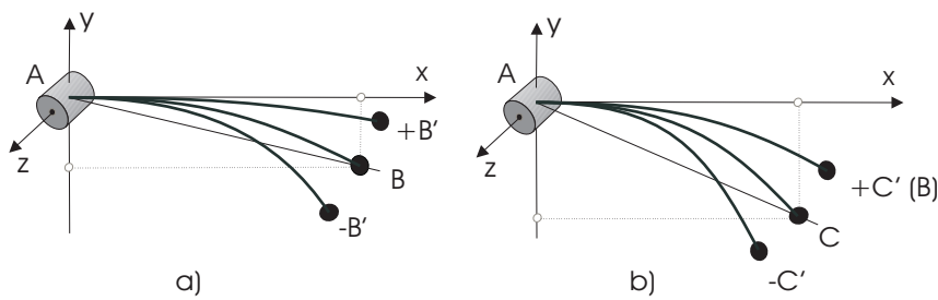
Figure 3: Stationary state position of a bending beam.
